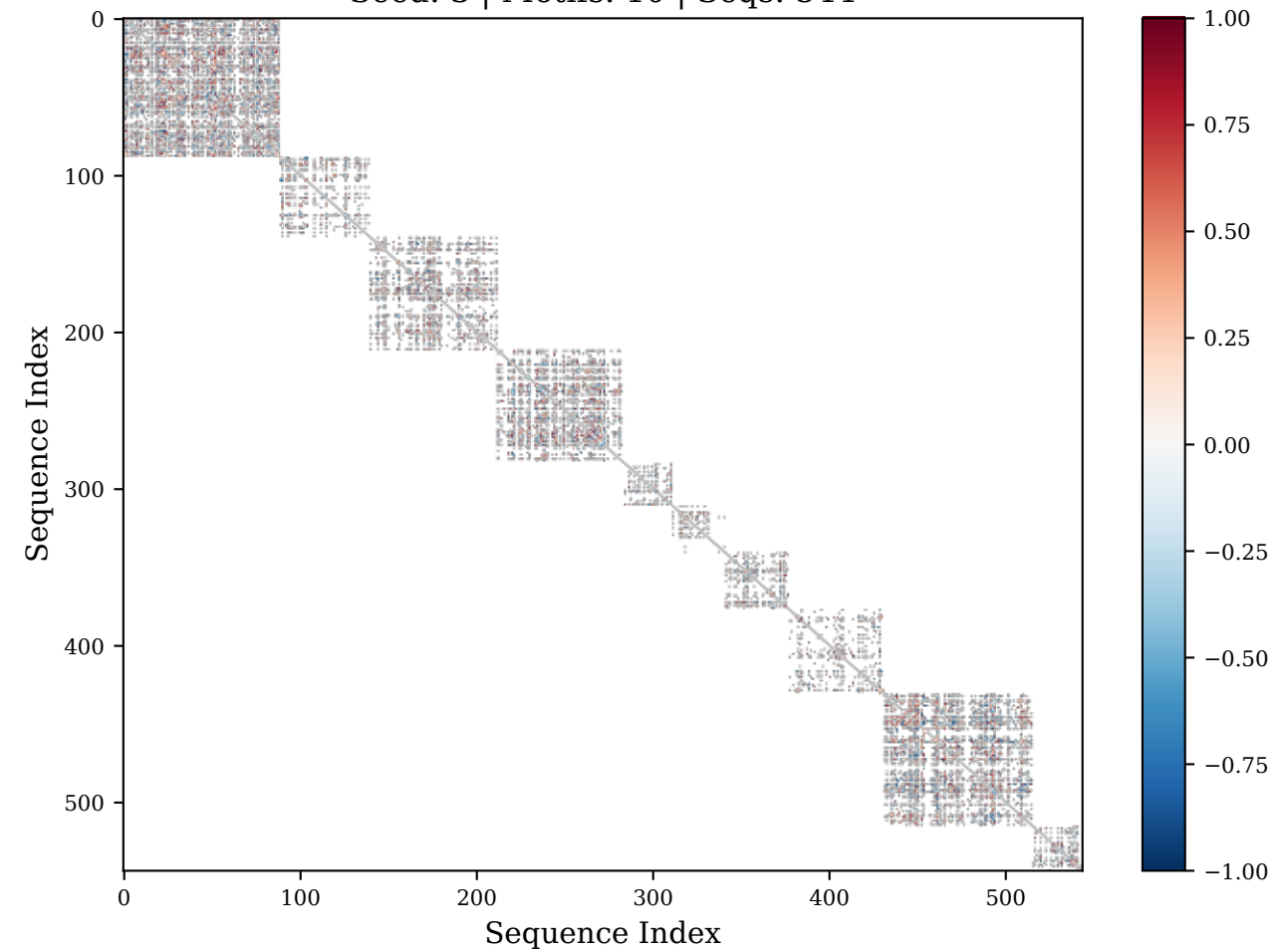
Seed: 3 | Motifs: 10 | Seqs: 544
