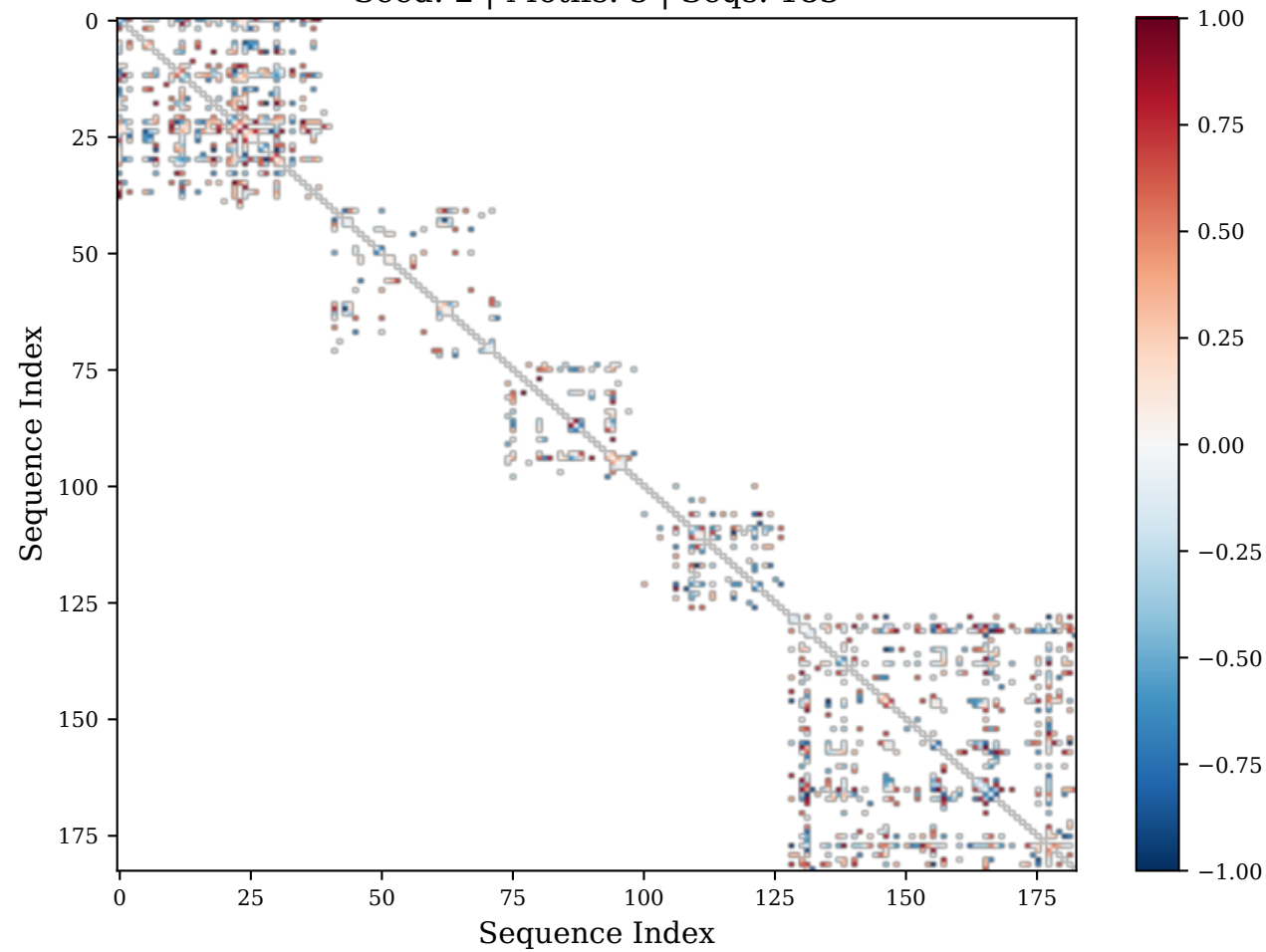
Seed: 2 | Motifs: 5 | Seqs: 183
